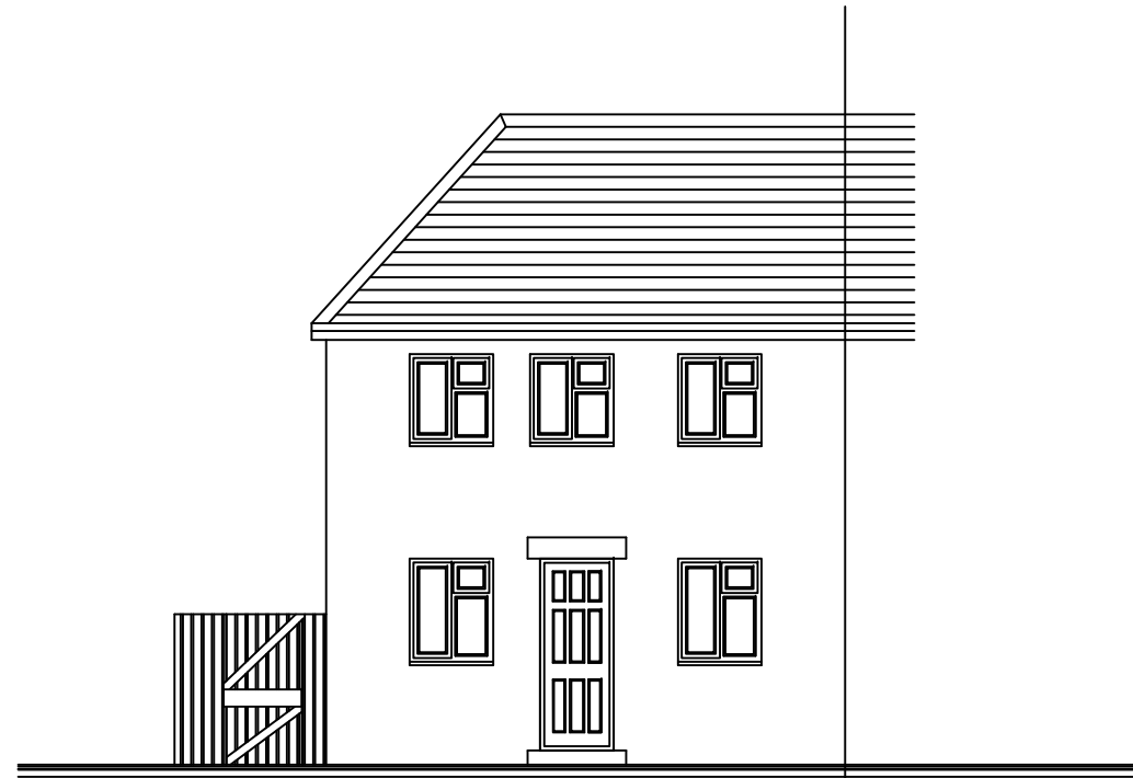
Back Elevation As Existing and Proposal House Itself.
